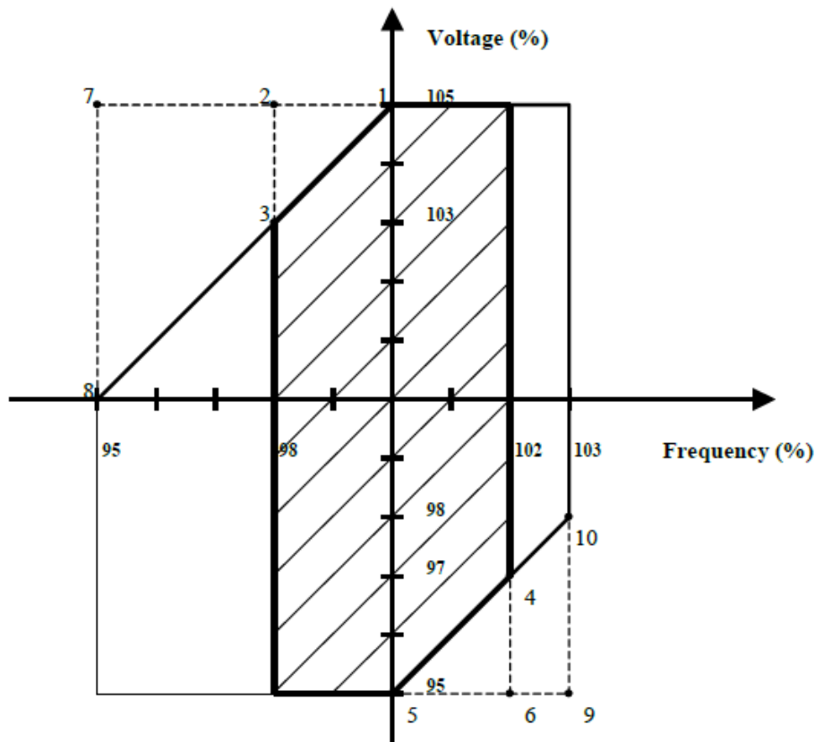
Figure 3-1: Transformer operating V/HZ curve
